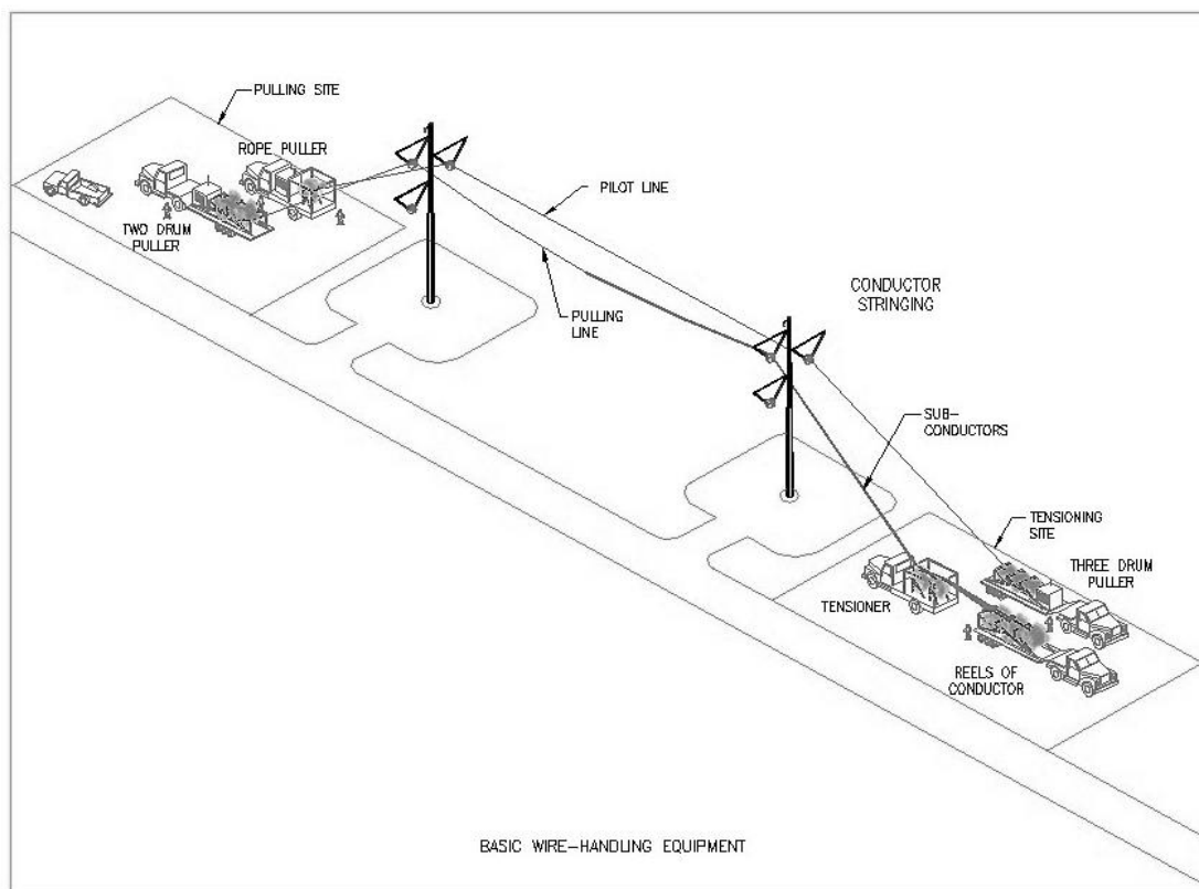
Figure 2-9. Typical Transmission Line Conductor Stringing Activities
